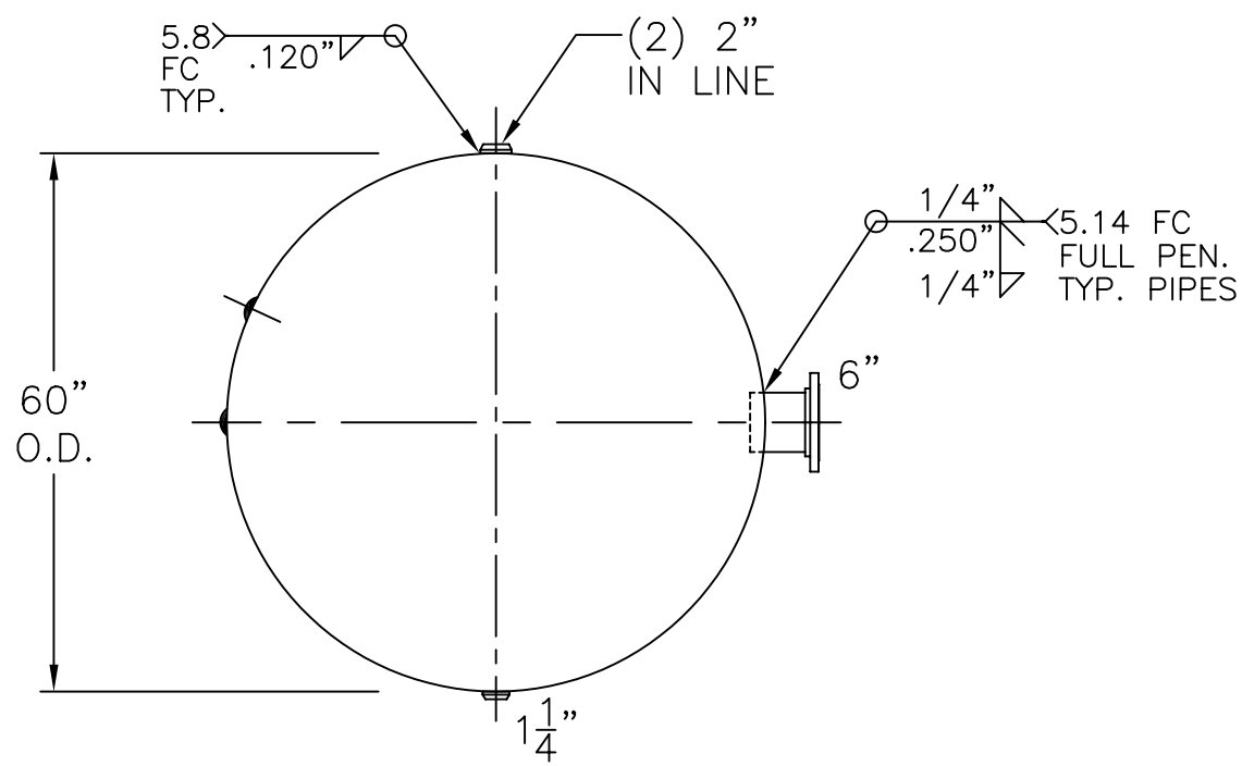
END VIEW W/OUT SUPT'S
